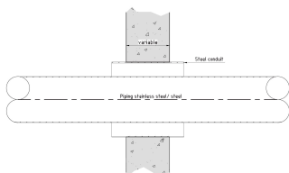
Sealing system for piping with or without steel conduit joint
